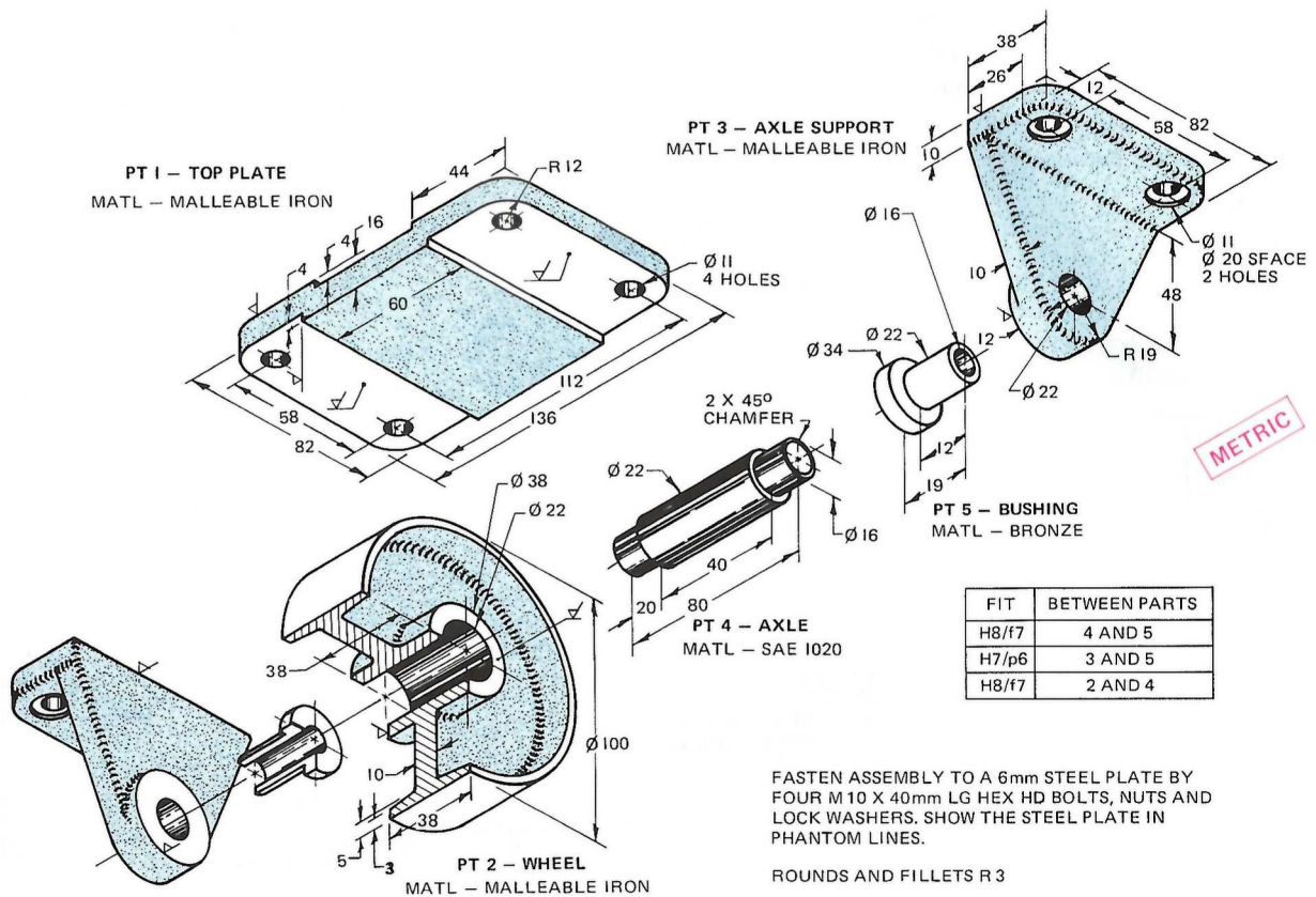
Fig. 9-51 Caster.
